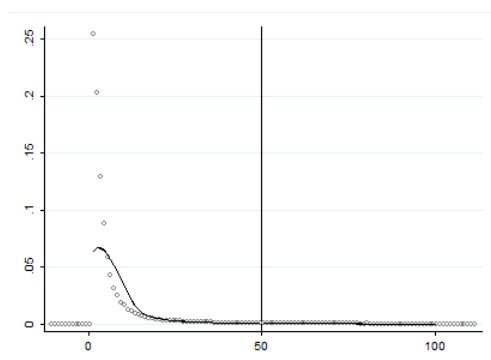
(c) McCrory Test (Before Logib)
