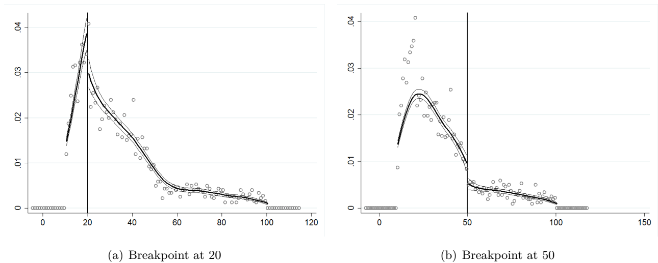
Figure 8: Graphical representation of McCrary Test with two breakpoints
