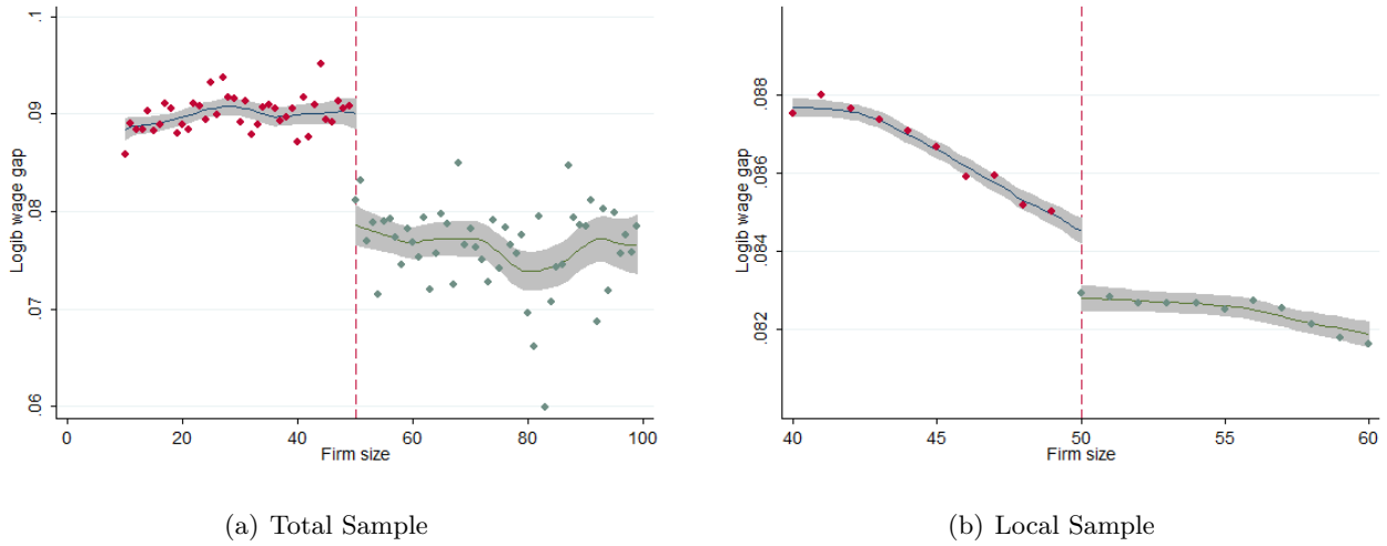
Figure 6: The effect of firm size on Logib wage gap after for the period between 2006-2010 Notes: Graphs are made using the total sample . Scatter points show the average of the mean gender coefficient by firm size. Solid lines refer to a third degree polynomial fit, and shadow area the 95% confidence interval of the fit. Reported graphs are shown in its simplest specification without considering controls variables. However, when considering big firms (with more than 250 workers), the industrial sector become more important, therefore RDD specifications for the Total sample include an additive dummy for the industrial sector.
